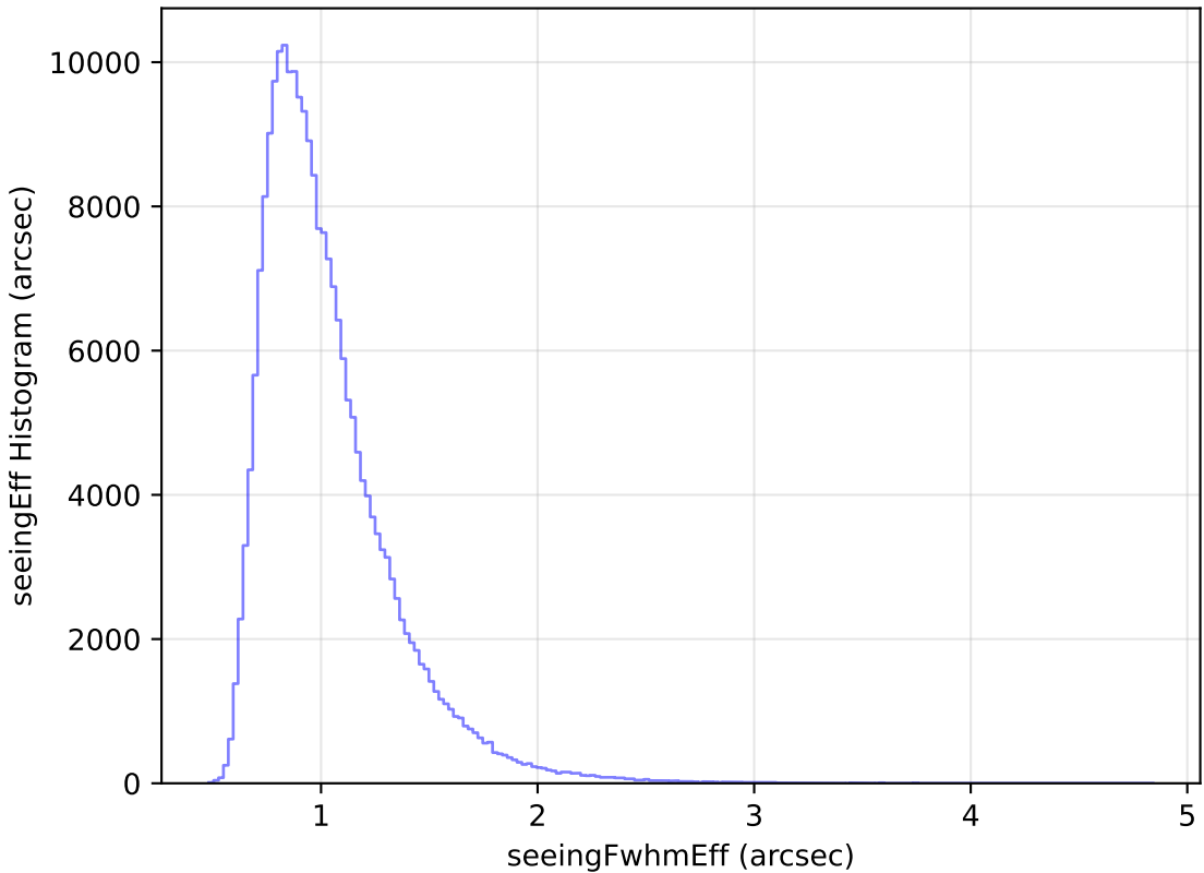
noroll_mjdp365_v3.4_10yrs Yr 1 all bands: seeingEff Histogram
