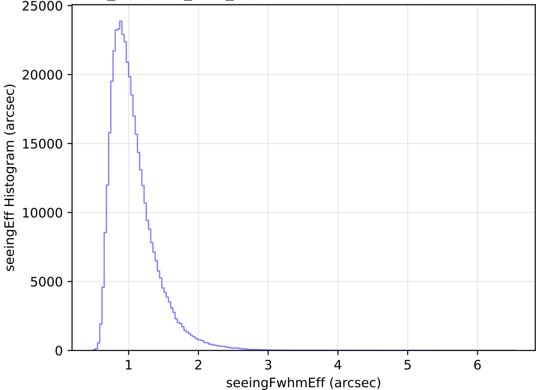
noroll_mjdp365_v3.4_10yrs WFD z band: seeingEff Histogram
