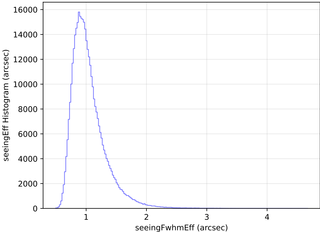
noroll_mjdp365_v3.4_10yrs WFD y band: seeingEff Histogram
