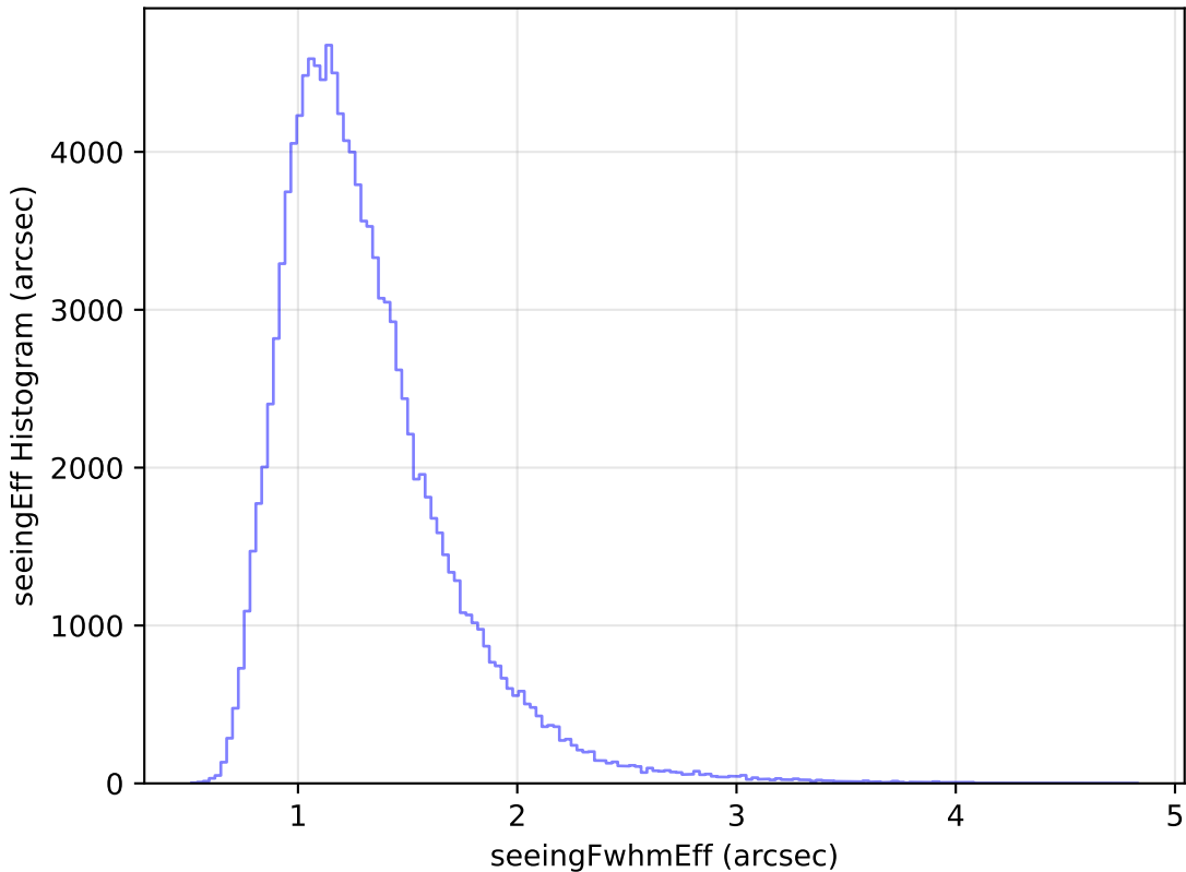
noroll_mjdp365_v3.4_10yrs WFD u band: seeingEff Histogram
