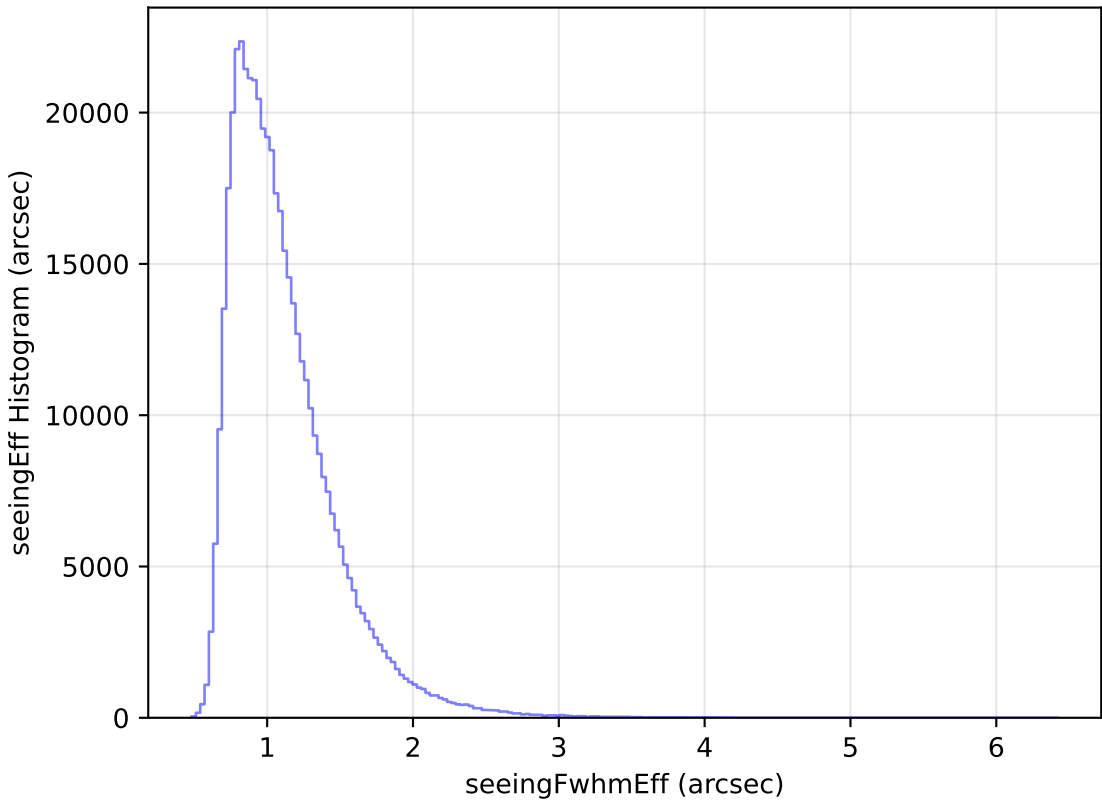
noroll_mjdp365_v3.4_10yrs WFD r band: seeingEff Histogram
