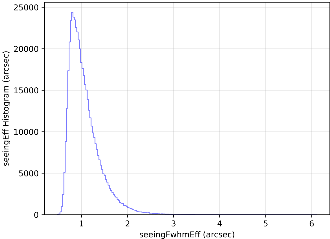
noroll_mjdp365_v3.4_10yrs WFD i band: seeingEff Histogram
