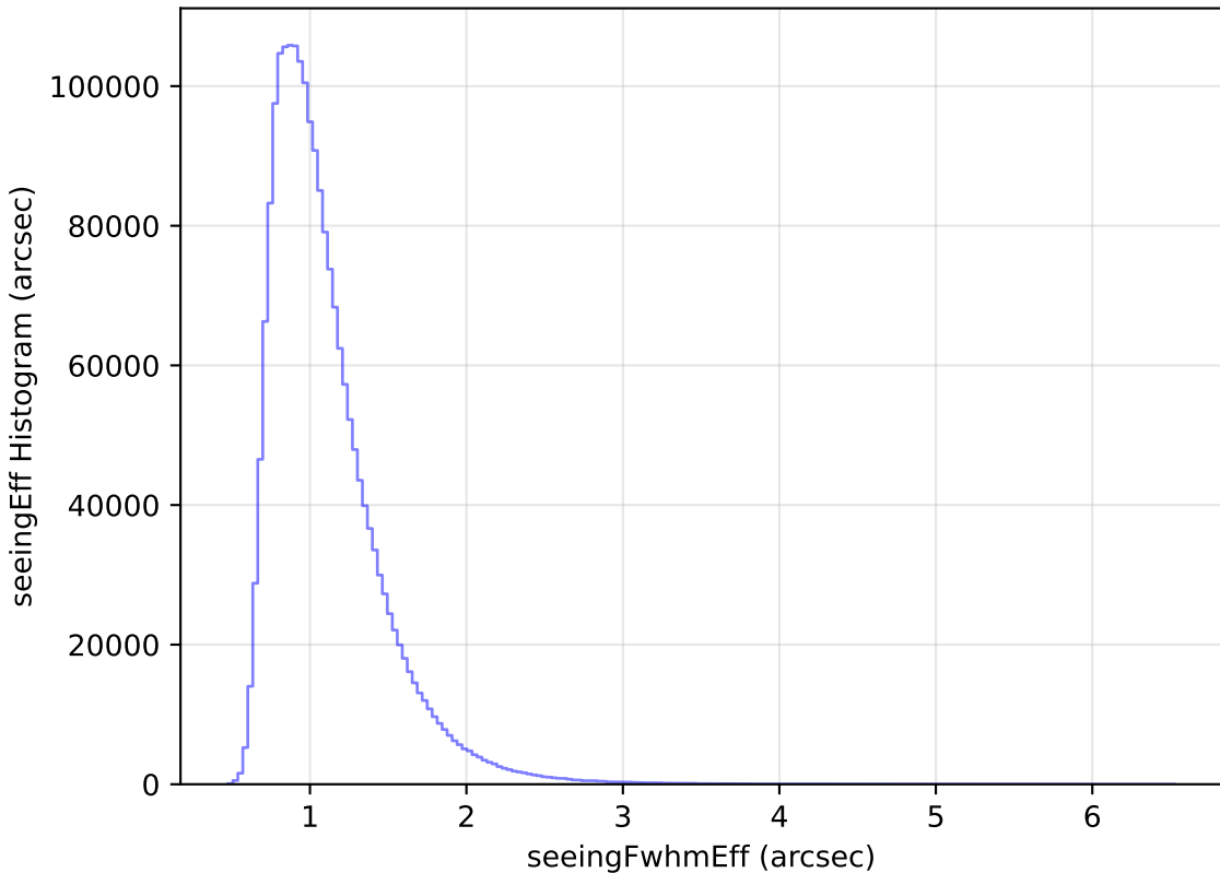
noroll_mjdp365_v3.4_10yrs WFD all bands: seeingEff Histogram
