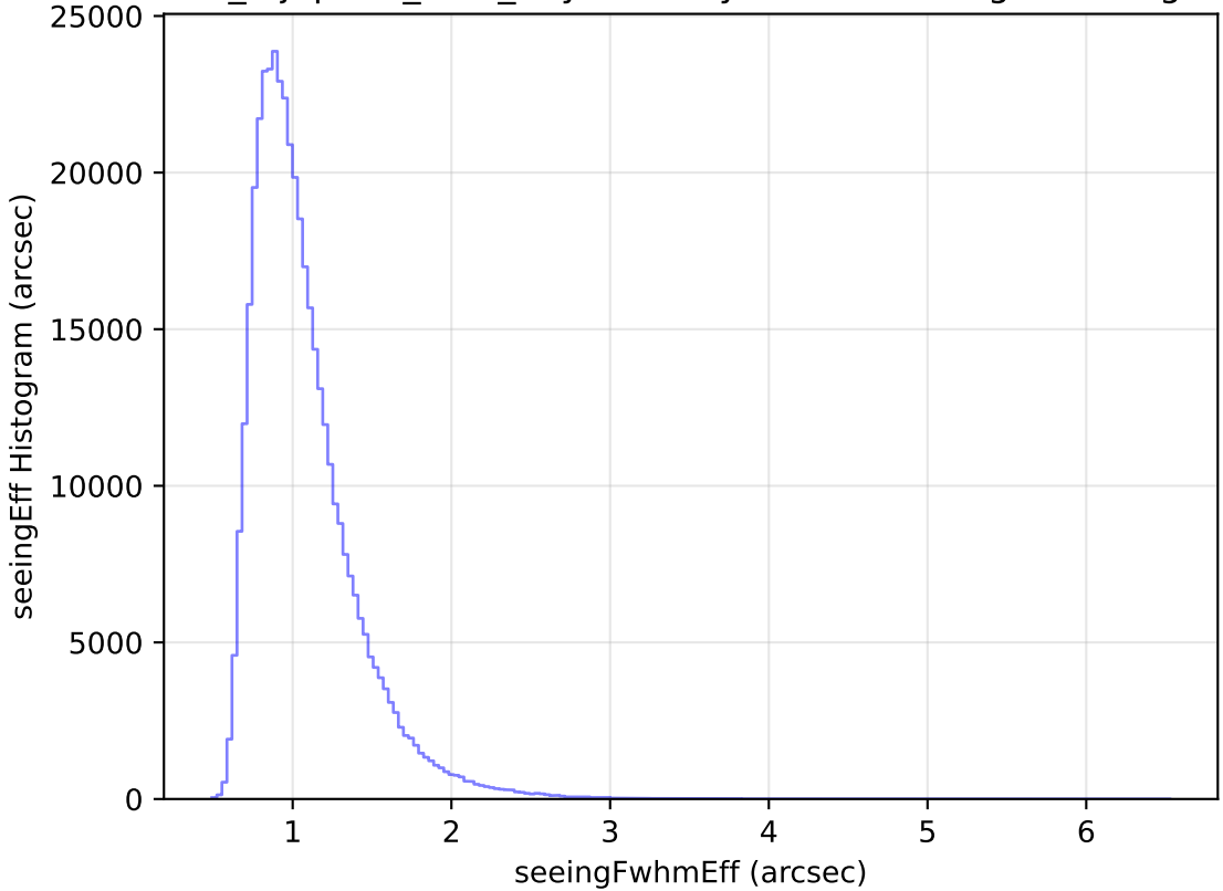
noroll_mjdp365_v3.4_10yrs All sky z band: seeingEff Histogram
