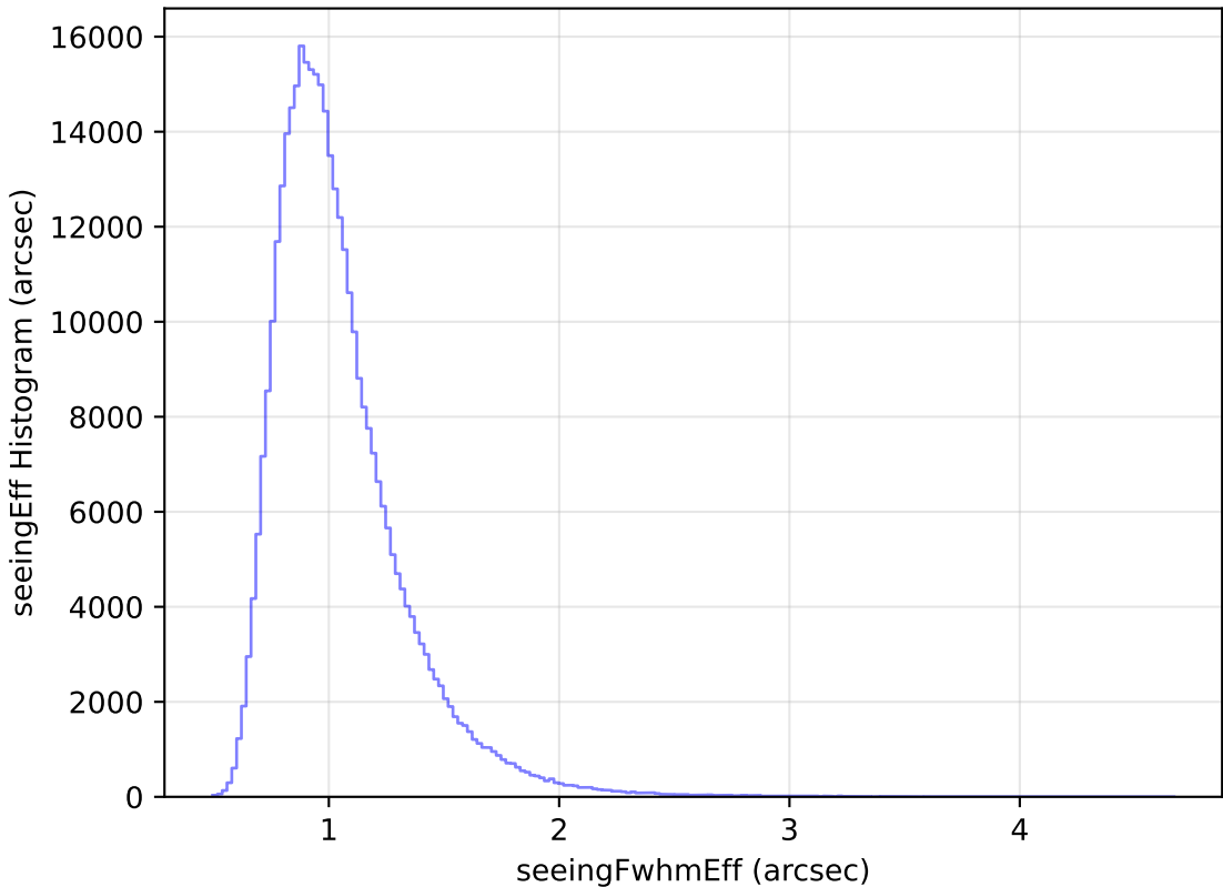
noroll_mjdp365_v3.4_10yrs All sky y band: seeingEff Histogram
