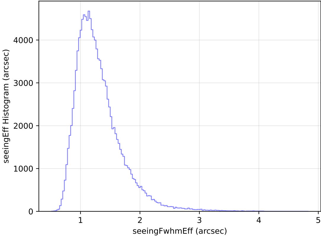
noroll_mjdp365_v3.4_10yrs All sky u band: seeingEff Histogram
