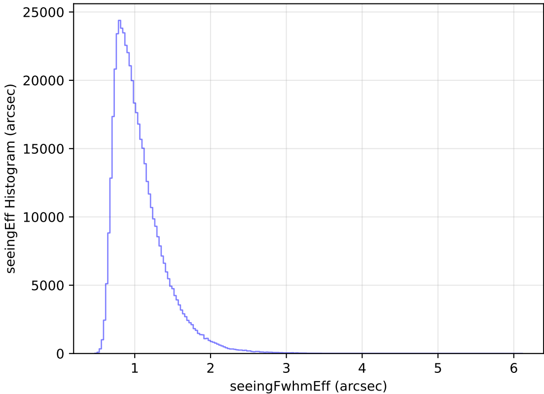
noroll_mjdp365_v3.4_10yrs All sky i band: seeingEff Histogram
