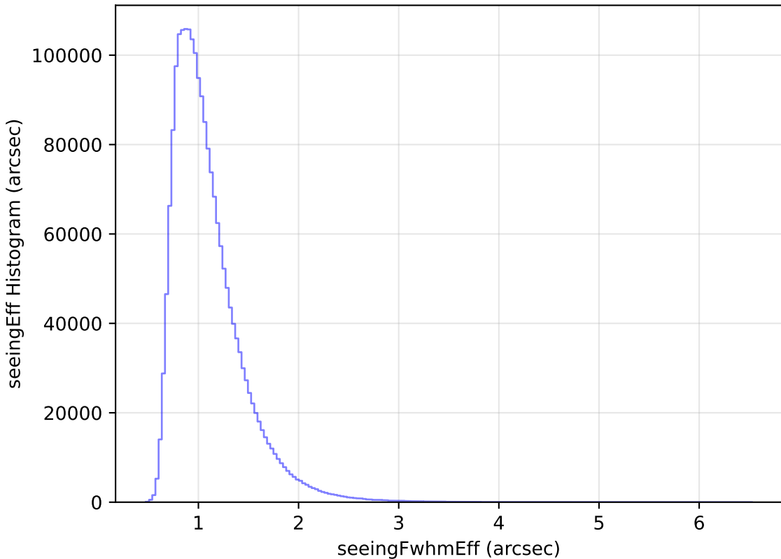
noroll_mjdp365_v3.4_10yrs All sky all bands: seeingEff Histogram
