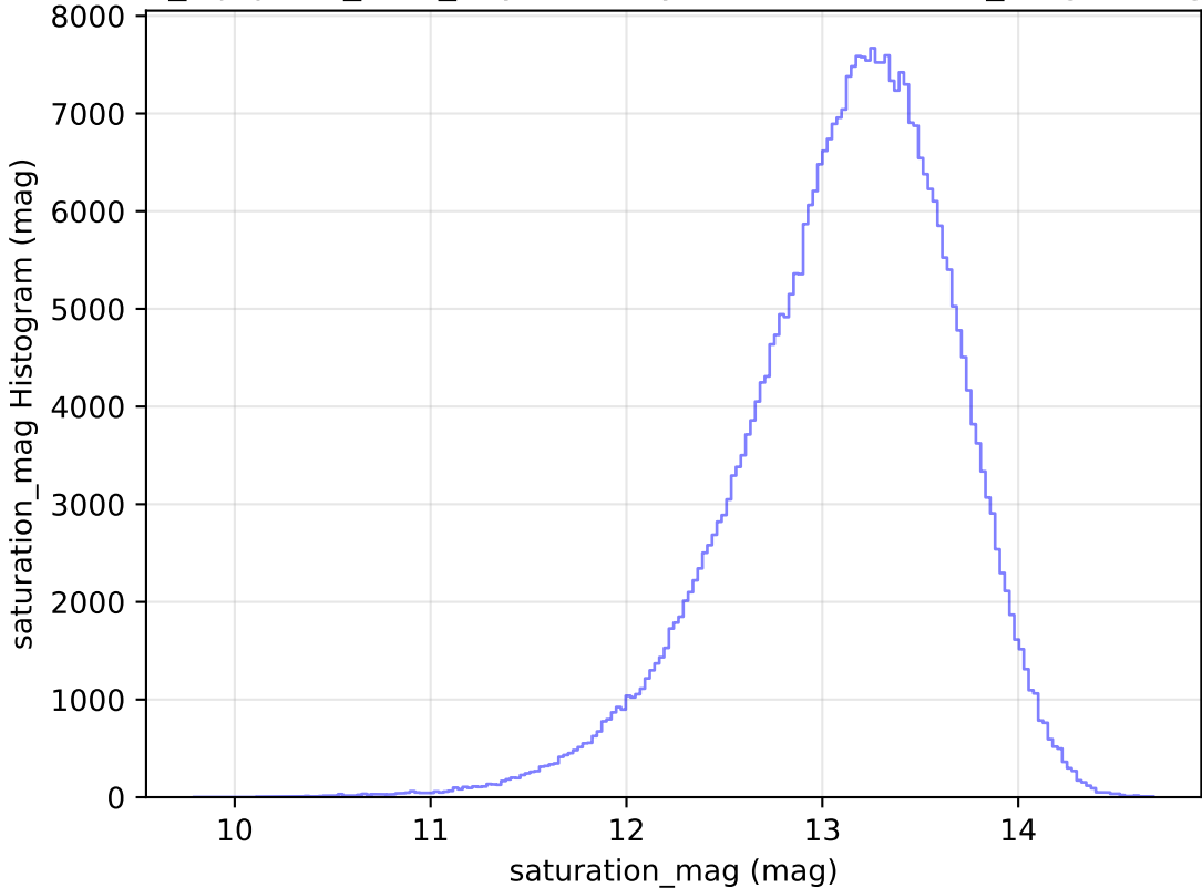
noroll_mjdp365_v3.4_10yrs WFD y band: saturation_mag Histogram
