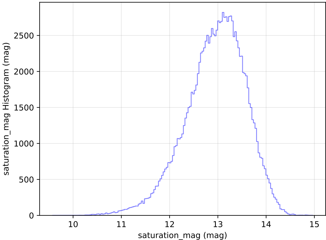
noroll_mjdp365_v3.4_10yrs WFD u band: saturation_mag Histogram
