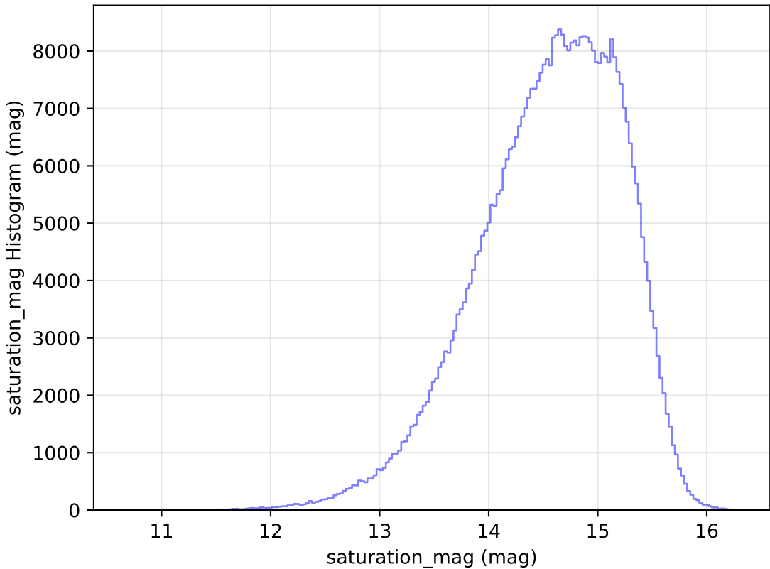
noroll_mjdp365_v3.4_10yrs WFD r band: saturation_mag Histogram
