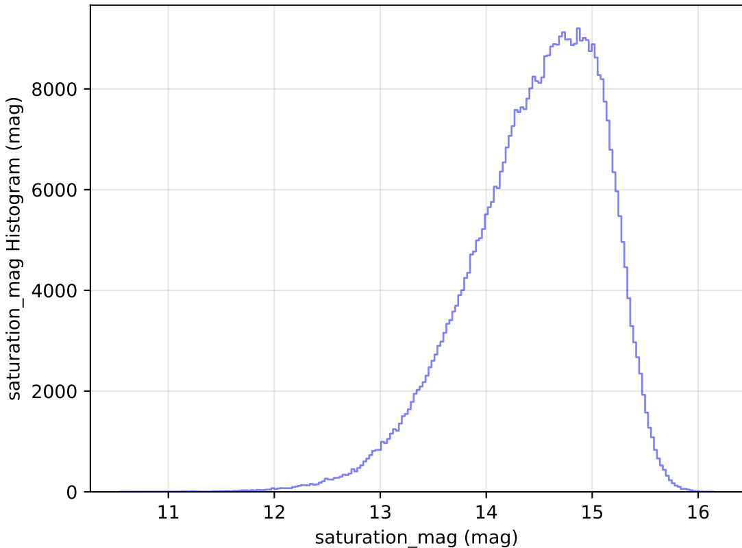
noroll_mjdp365_v3.4_10yrs WFD i band: saturation_mag Histogram
