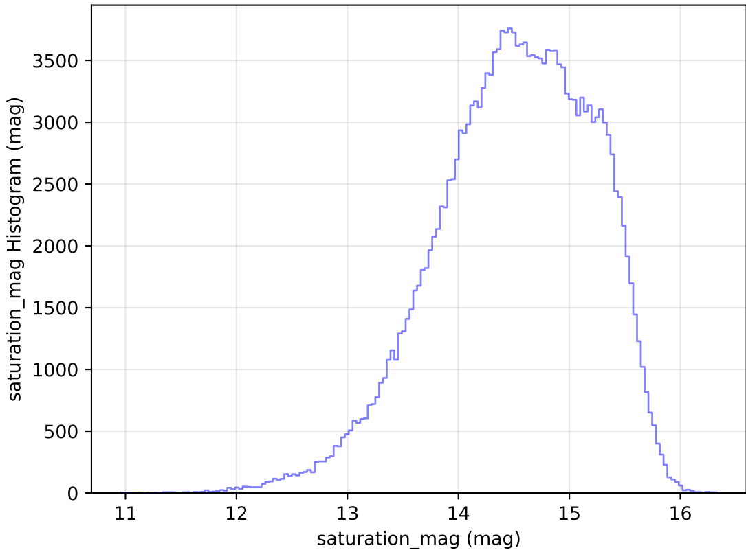
noroll_mjdp365_v3.4_10yrs WFD g band: saturation_mag Histogram
