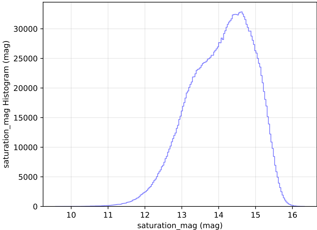
noroll_mjdp365_v3.4_10yrs WFD all bands: saturation_mag Histogram
