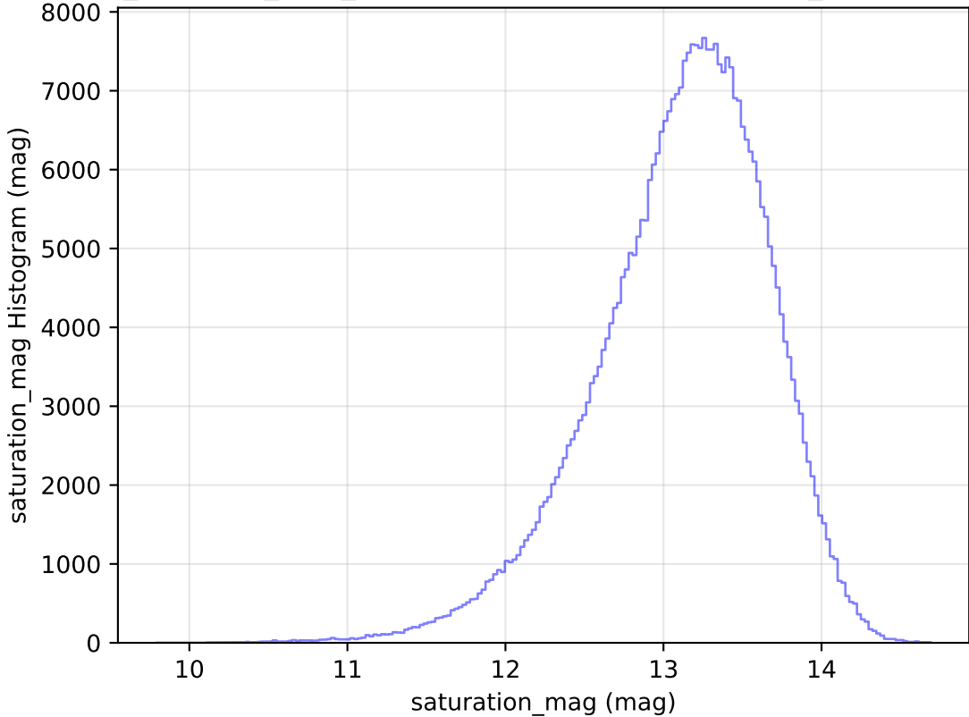
noroll_mjdp365_v3.4_10yrs All sky y band: saturation_mag Histogram
