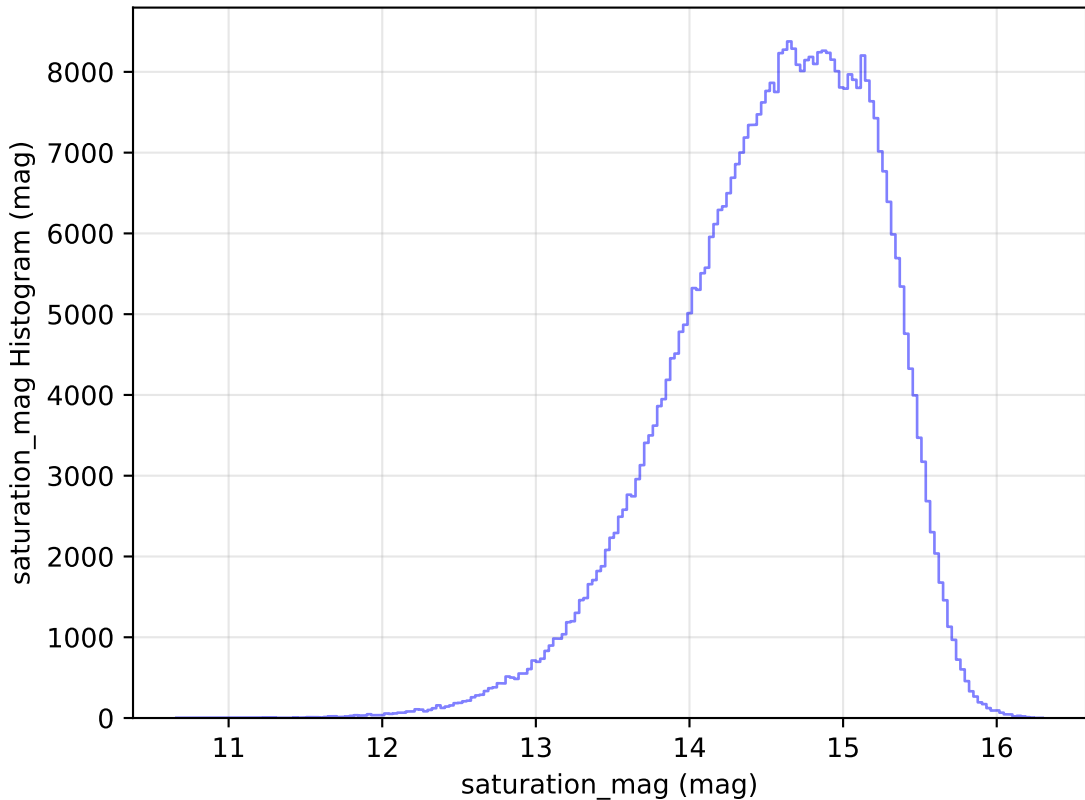
noroll_mjdp365_v3.4_10yrs All sky r band: saturation_mag Histogram
