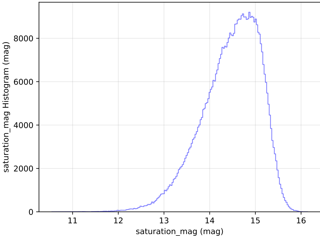
noroll_mjdp365_v3.4_10yrs All sky i band: saturation_mag Histogram
