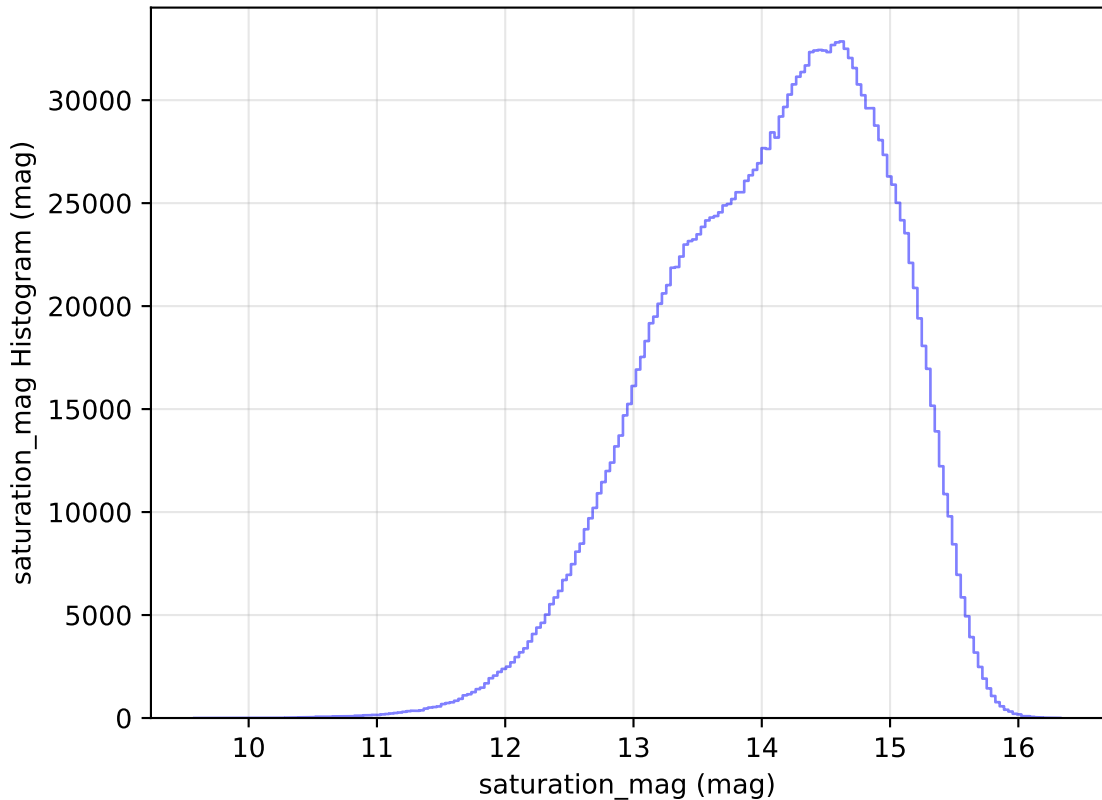
noroll_mjdp365_v3.4_10yrs All sky all bands: saturation_mag Histogram
