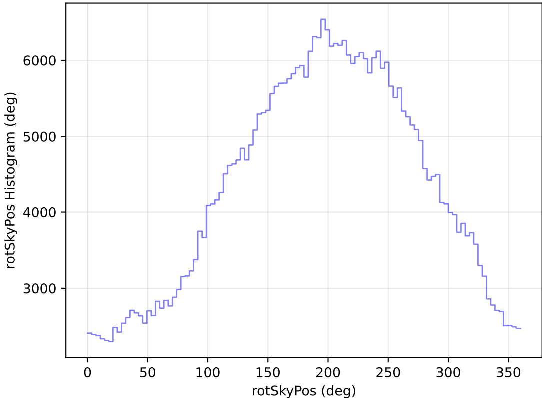
noroll_mjdp365_v3.4_10yrs WFD z band: rotSkyPos Histogram
