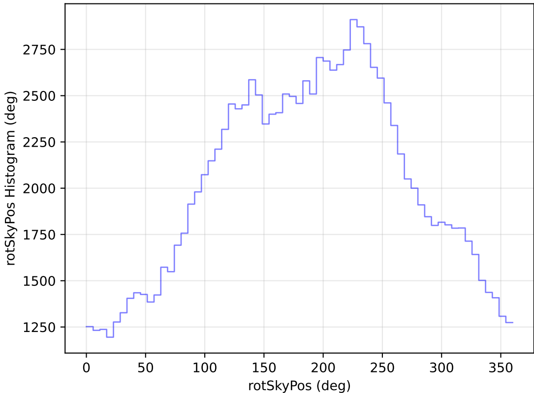
noroll_mjdp365_v3.4_10yrs WFD u band: rotSkyPos Histogram
