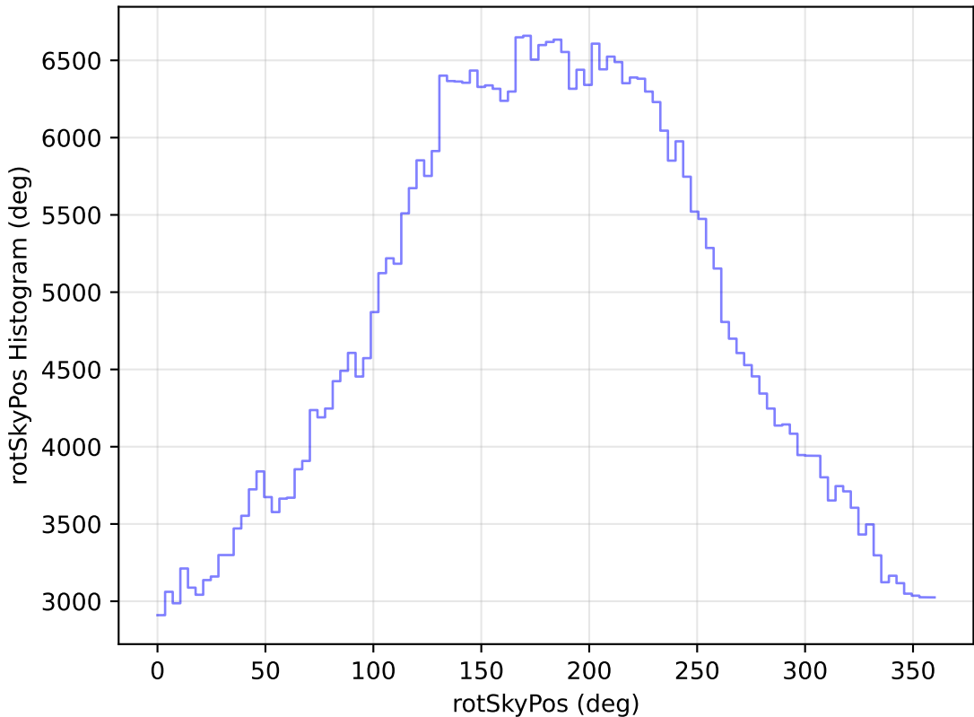
noroll_mjdp365_v3.4_10yrs WFD r band: rotSkyPos Histogram
