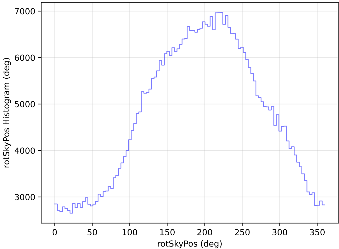
noroll_mjdp365_v3.4_10yrs WFD i band: rotSkyPos Histogram
