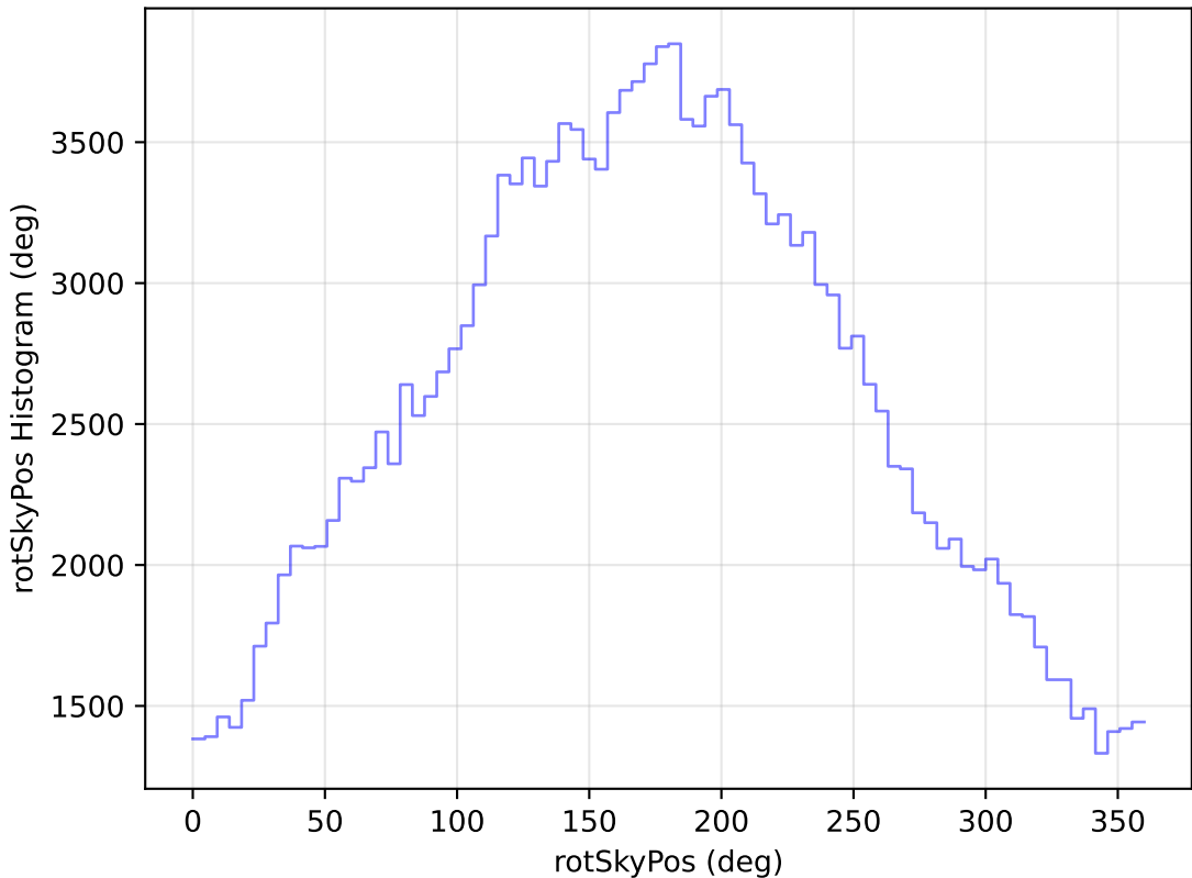
noroll_mjdp365_v3.4_10yrs WFD g band: rotSkyPos Histogram
