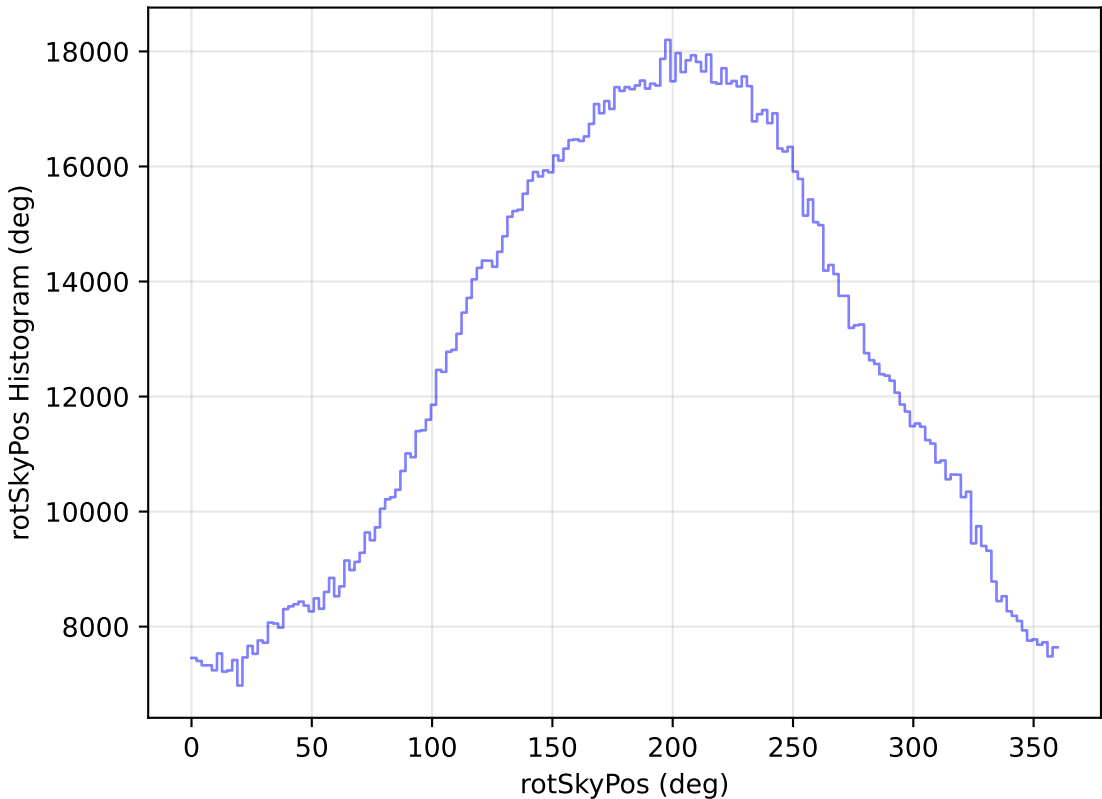
noroll_mjdp365_v3.4_10yrs WFD all bands: rotSkyPos Histogram
