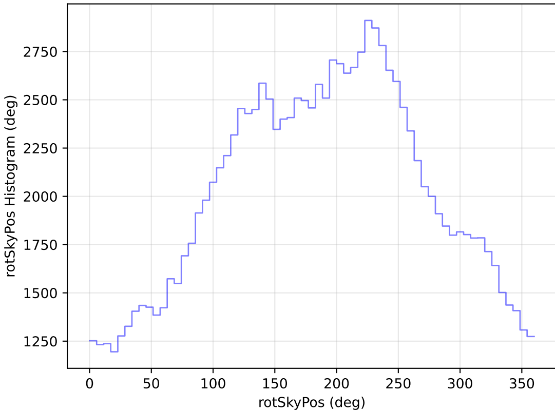
noroll_mjdp365_v3.4_10yrs All sky u band: rotSkyPos Histogram
