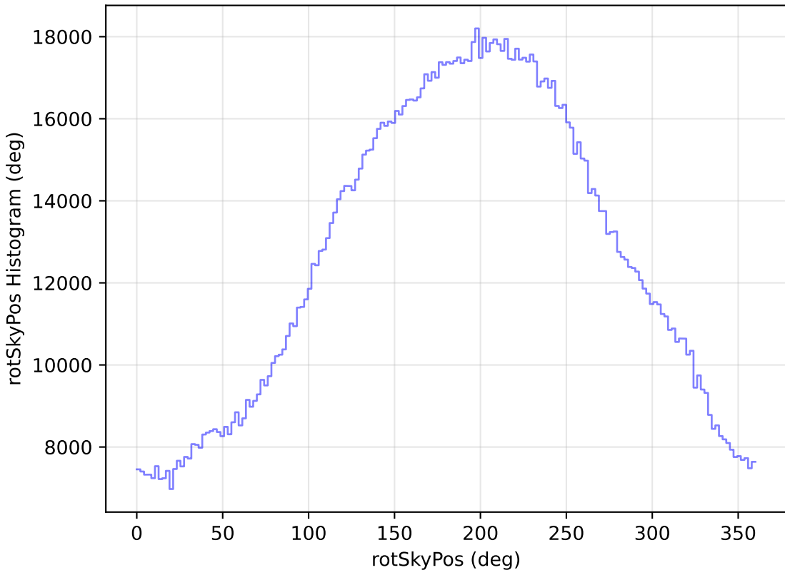
noroll_mjdp365_v3.4_10yrs All sky all bands: rotSkyPos Histogram
