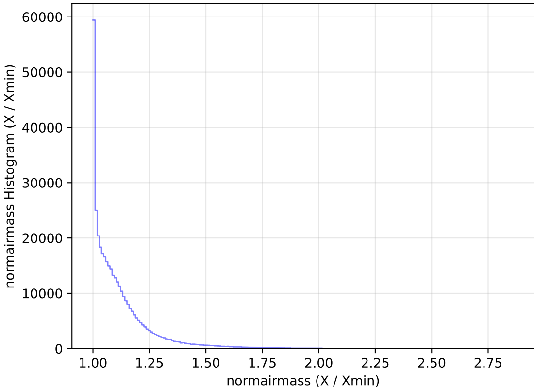
noroll_mjdp365_v3.4_10yrs WFD y band: normairmass Histogram
