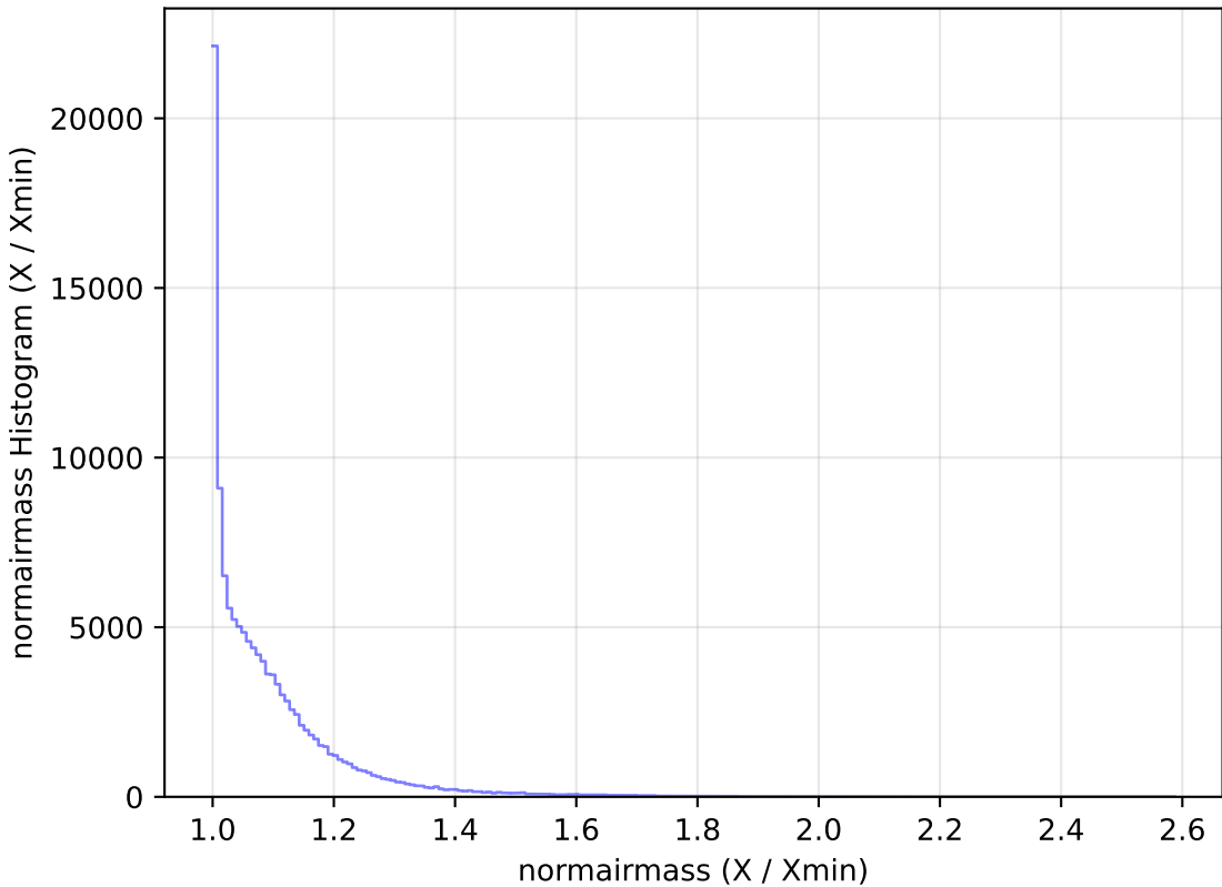
noroll_mjdp365_v3.4_10yrs WFD u band: normairmass Histogram
