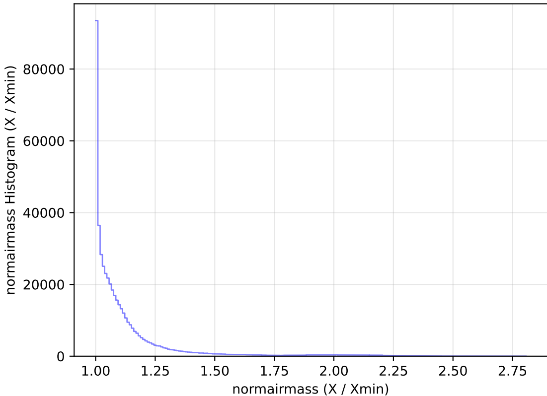
noroll_mjdp365_v3.4_10yrs WFD r band: normairmass Histogram
