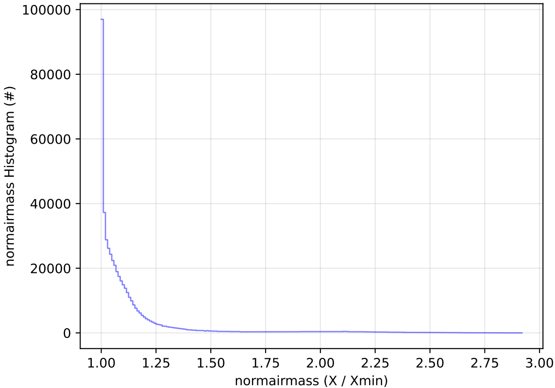
noroll_mjdp365_v3.4_10yrs WFD i band: normairmass Histogram
