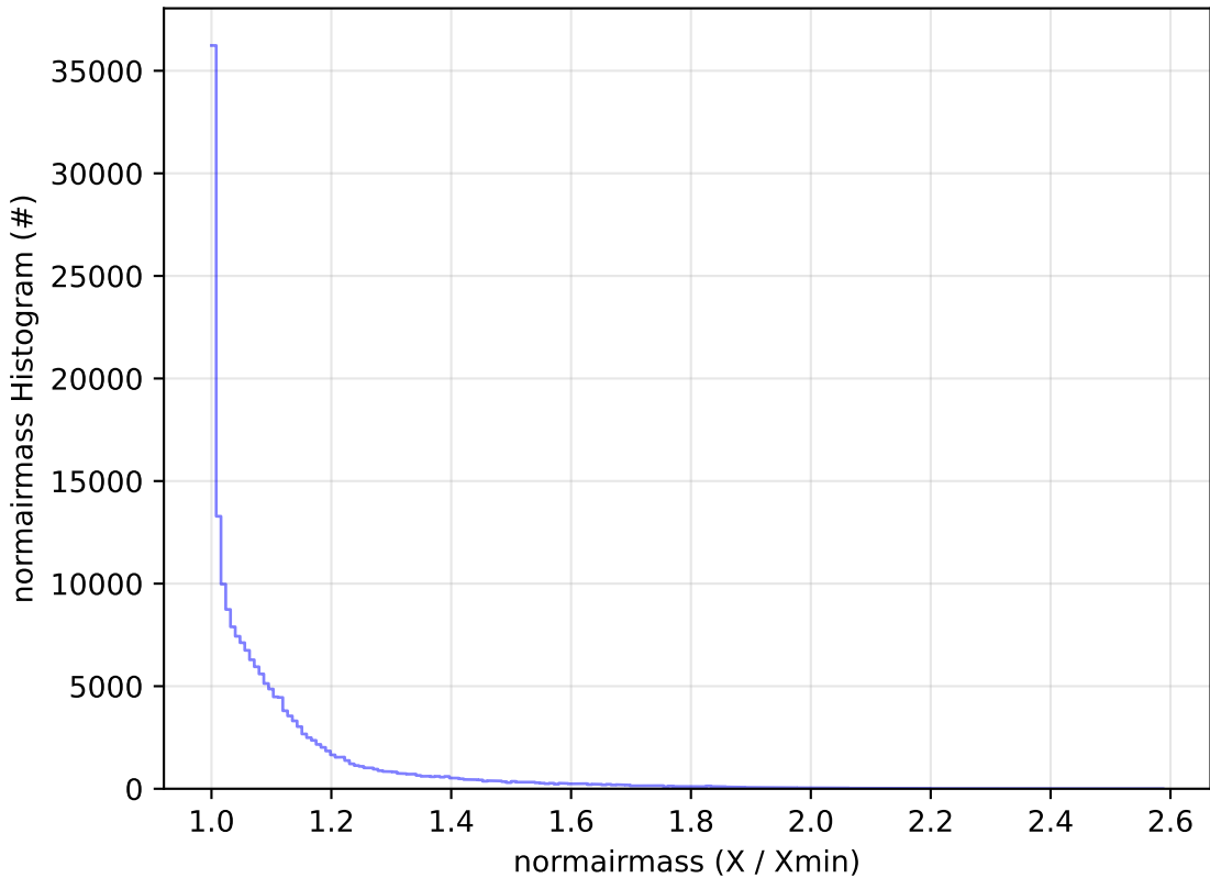
noroll_mjdp365_v3.4_10yrs WFD g band: normairmass Histogram
