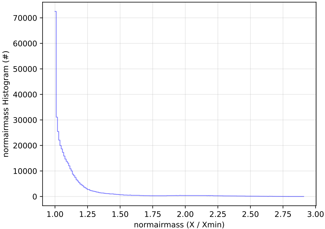
noroll_mjdp365_v3.4_10yrs All sky z band: normairmass Histogram
