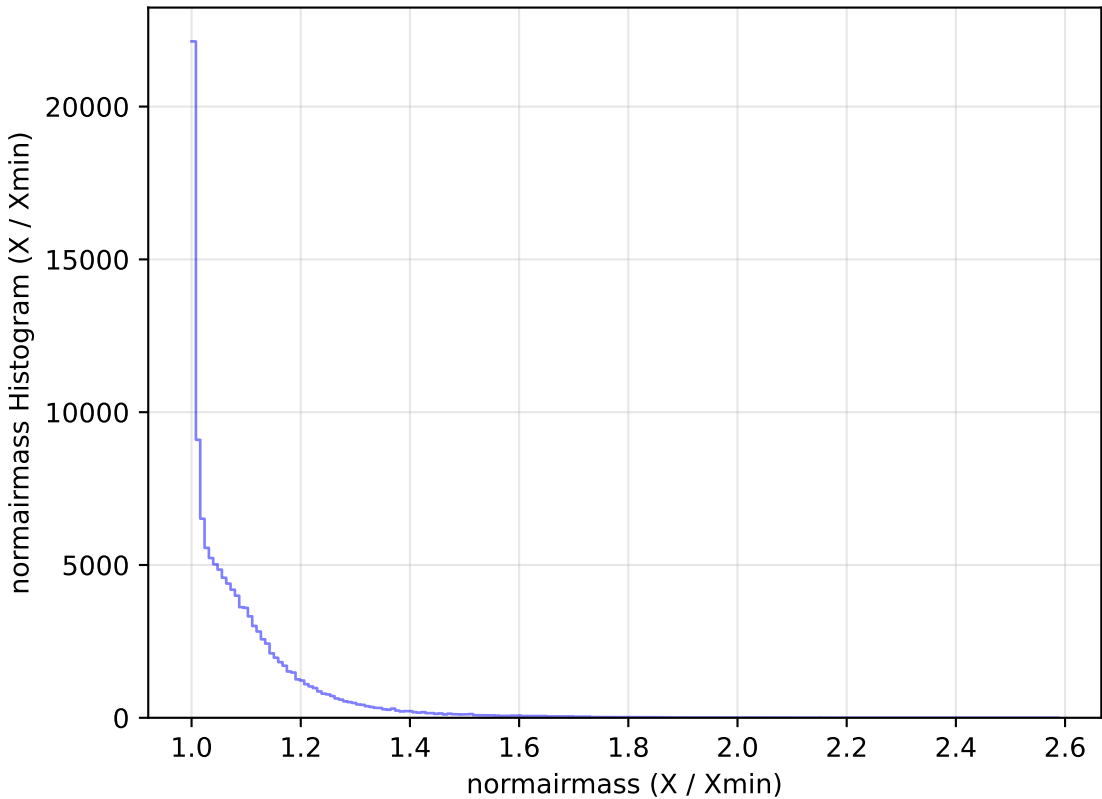
noroll_mjdp365_v3.4_10yrs All sky u band: normairmass Histogram
