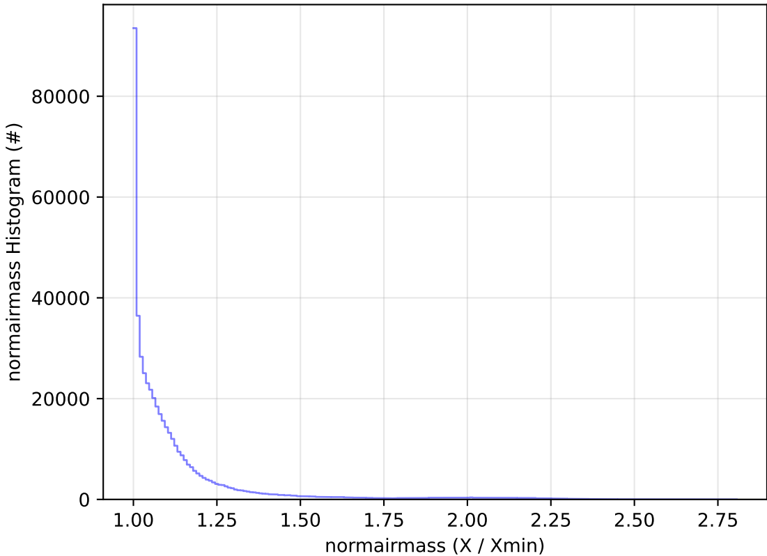
noroll_mjdp365_v3.4_10yrs All sky r band: normairmass Histogram
