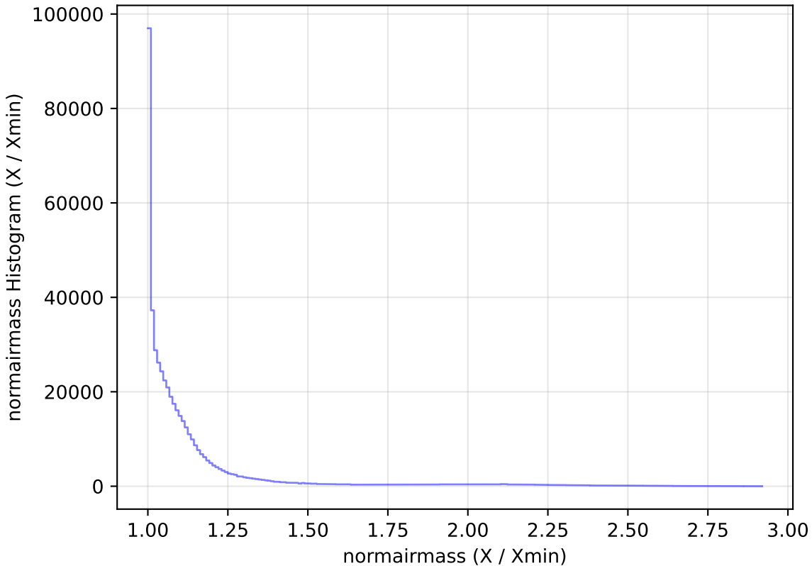
noroll_mjdp365_v3.4_10yrs All sky i band: normairmass Histogram
