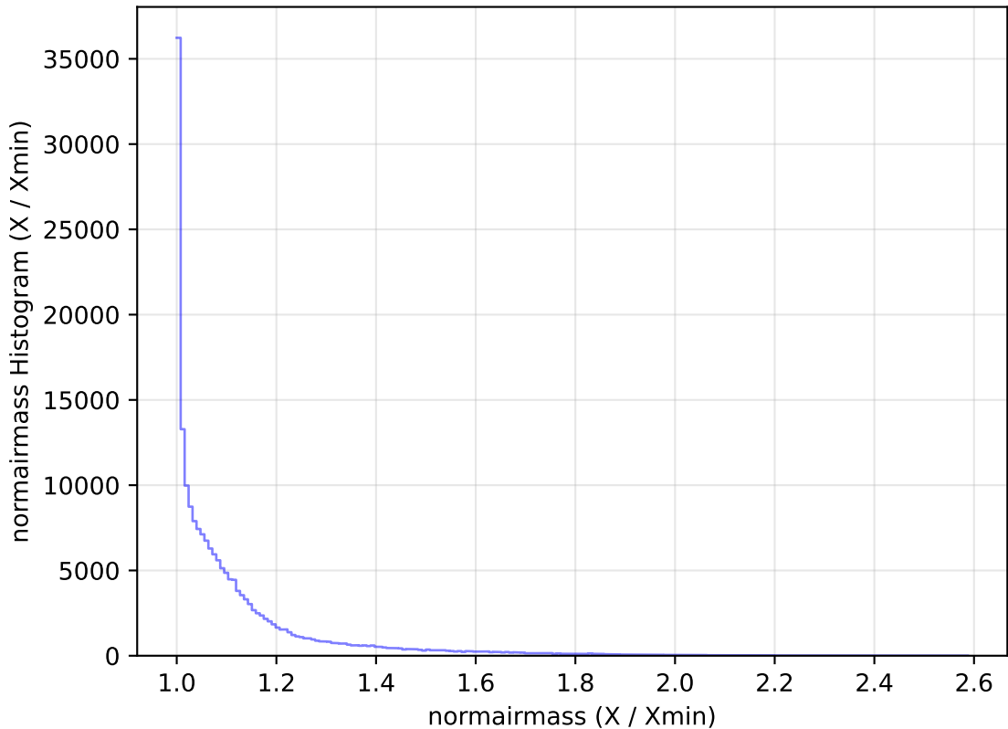
noroll_mjdp365_v3.4_10yrs All sky g band: normairmass Histogram
