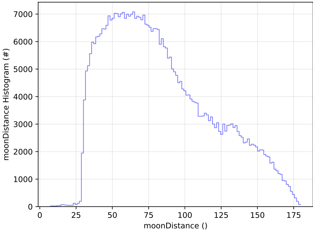
noroll_mjdp365_v3.4_10yrs WFD z band: moonDistance Histogram
