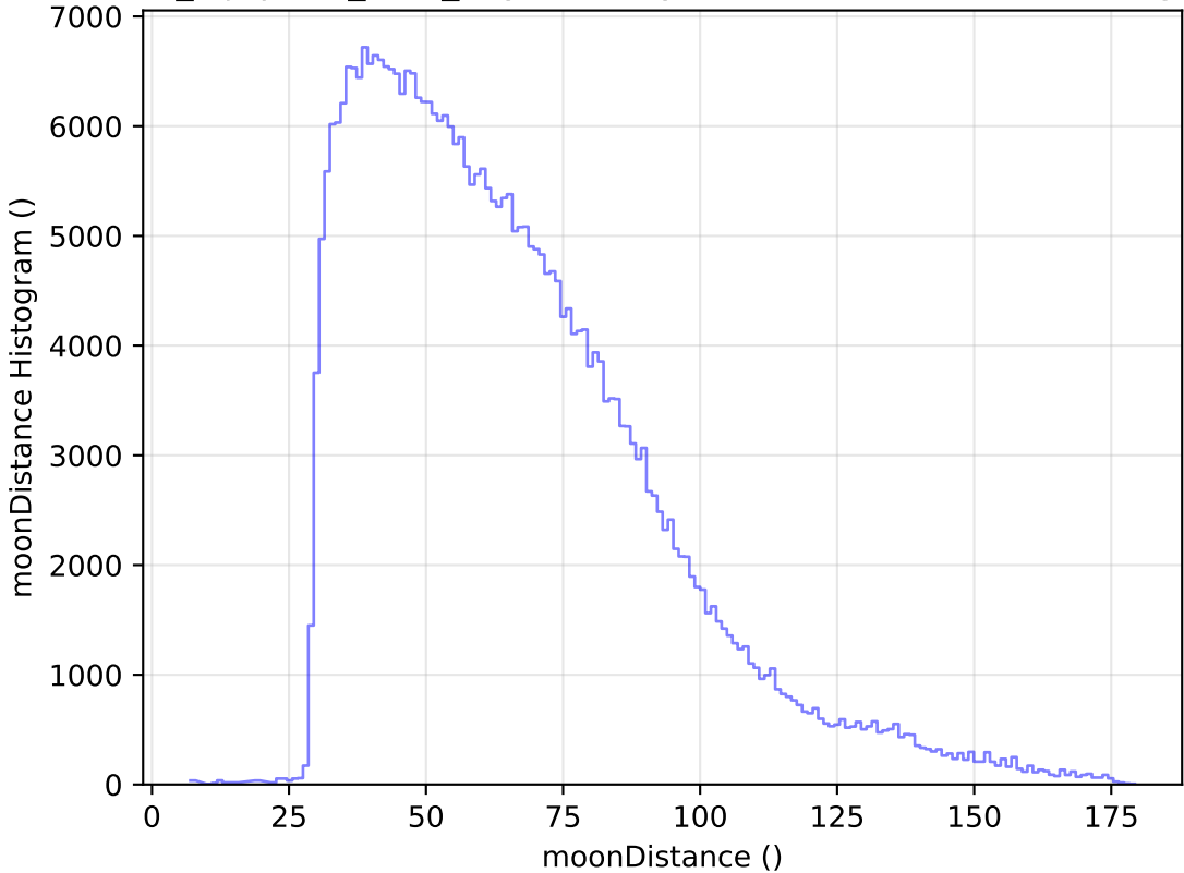
noroll_mjdp365_v3.4_10yrs WFD y band: moonDistance Histogram
