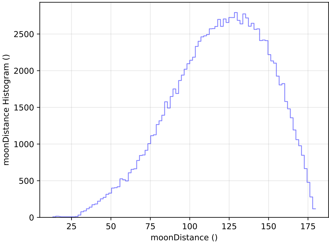
noroll_mjdp365_v3.4_10yrs WFD u band: moonDistance Histogram
