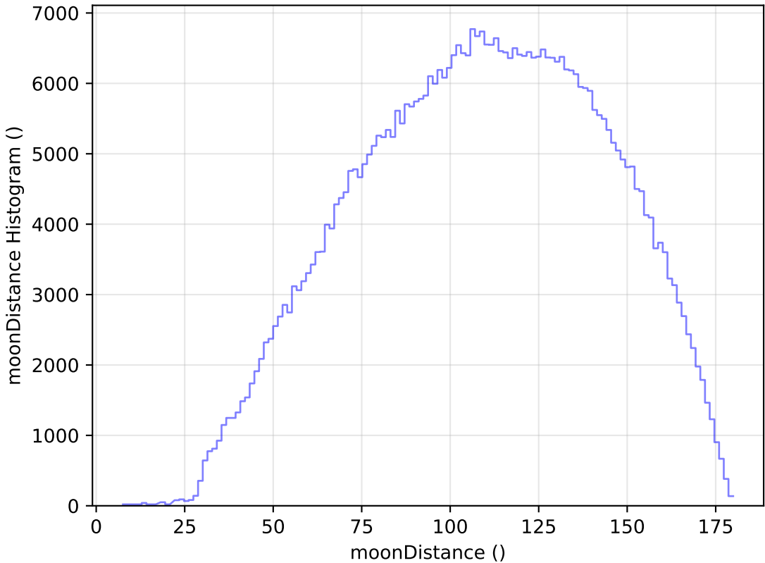
noroll_mjdp365_v3.4_10yrs WFD r band: moonDistance Histogram
