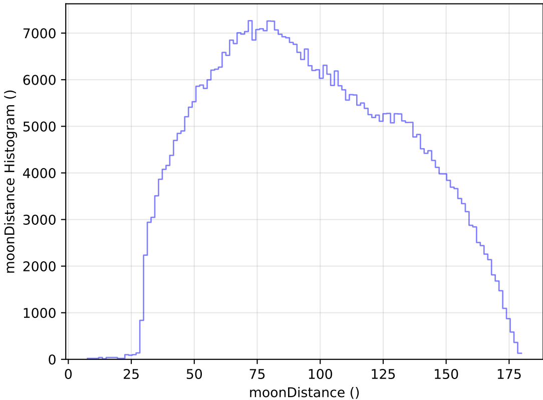
noroll_mjdp365_v3.4_10yrs WFD i band: moonDistance Histogram
