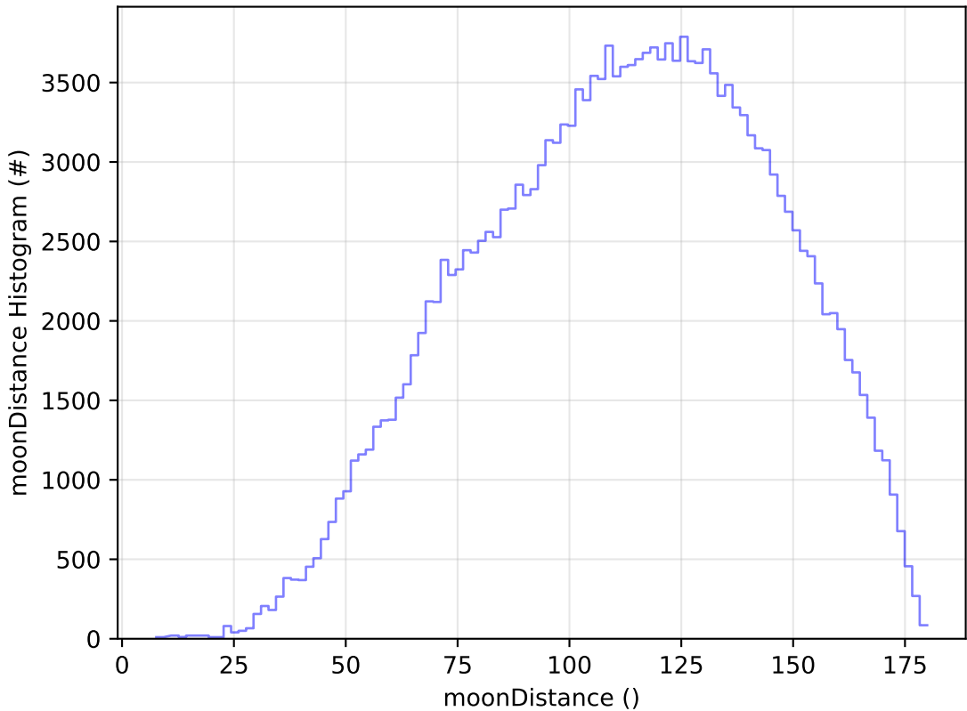
noroll_mjdp365_v3.4_10yrs WFD g band: moonDistance Histogram
