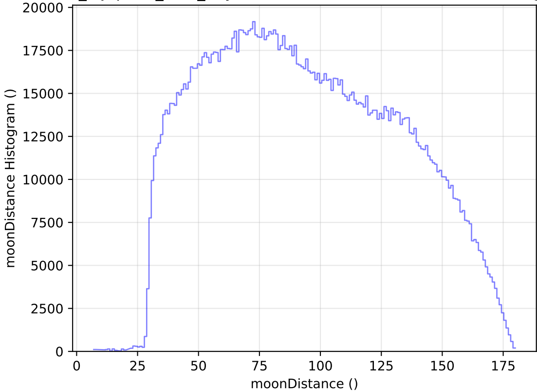
noroll_mjdp365_v3.4_10yrs WFD all bands: moonDistance Histogram
