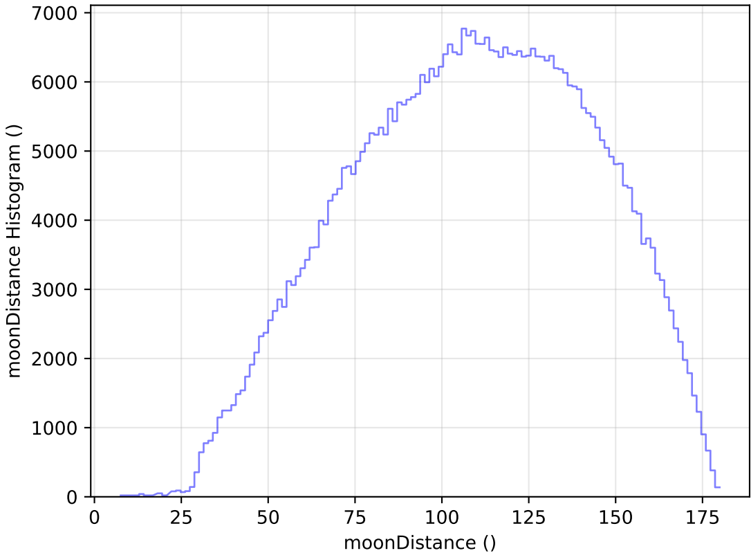
noroll_mjdp365_v3.4_10yrs All sky r band: moonDistance Histogram
