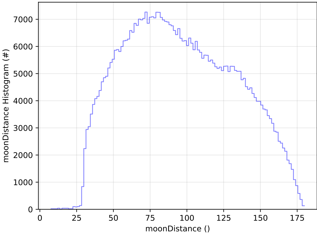
noroll_mjdp365_v3.4_10yrs All sky i band: moonDistance Histogram
