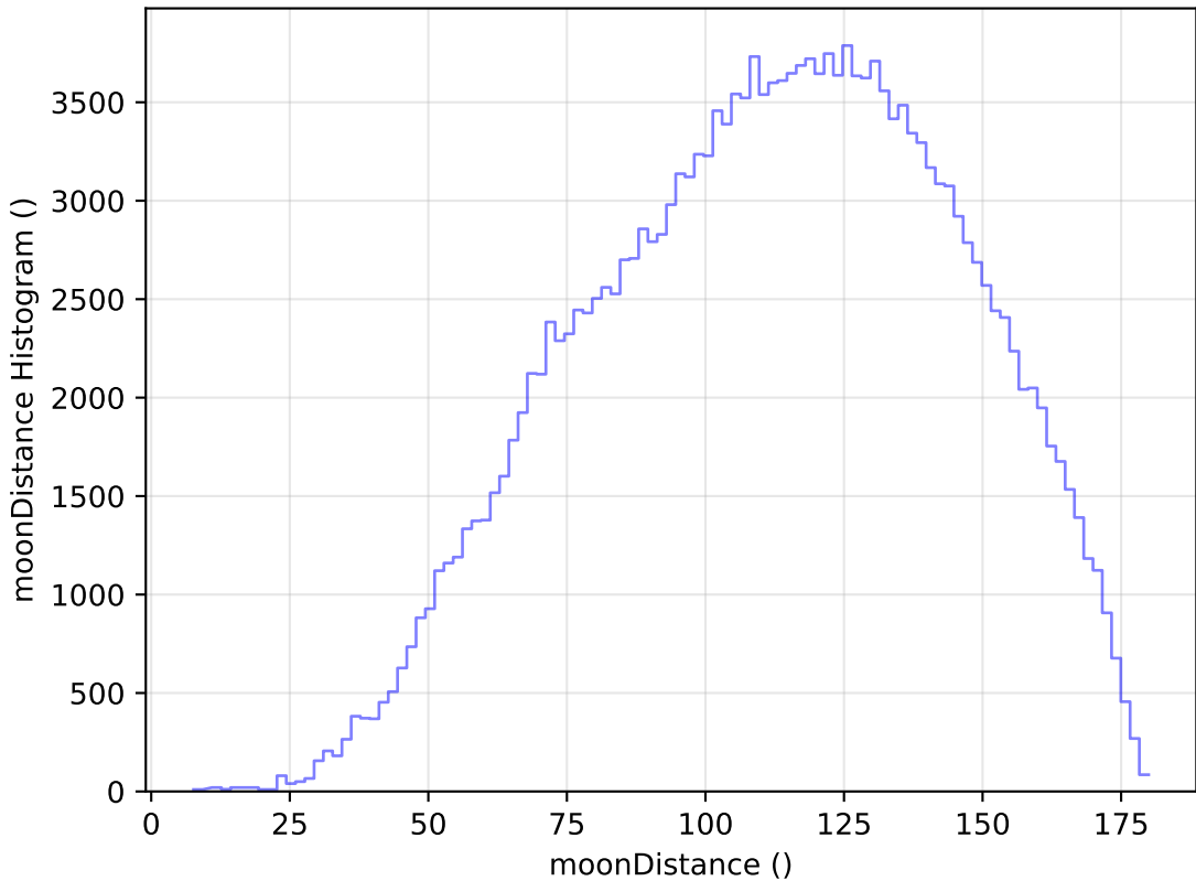
noroll_mjdp365_v3.4_10yrs All sky g band: moonDistance Histogram
